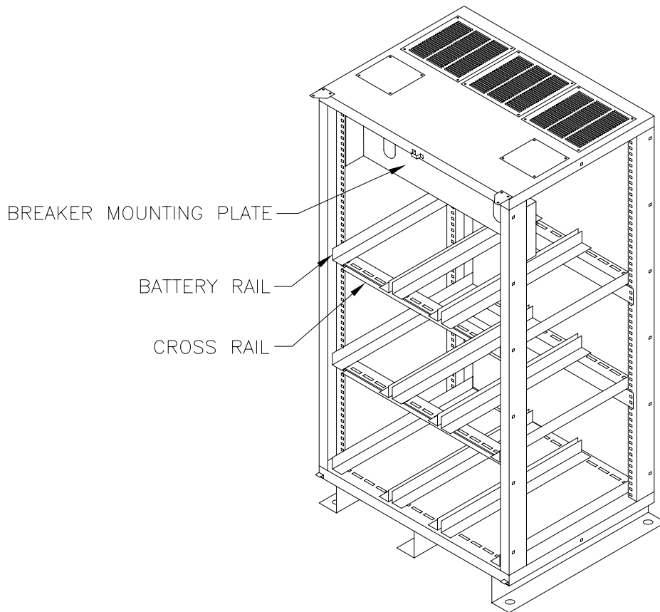
VITALSINE BASE CABINET, BATTERY CABINET CONFIGURATION
