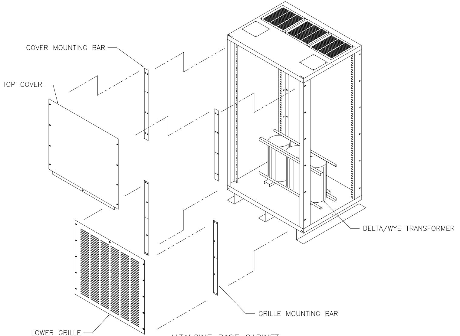
VITALSINE BASE CABINET, INPUT CABINET CONFIGURATION
