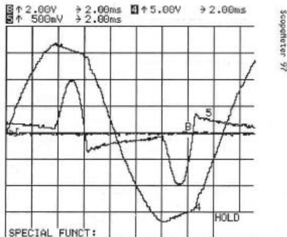
Figure 1 – Voltage vs. Current in SMPS
