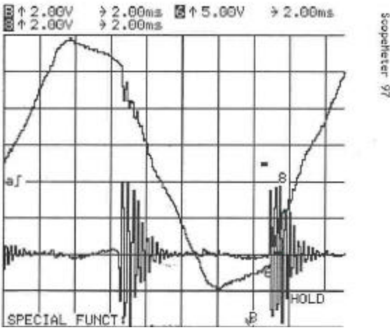
Figure 3 Normal Mode Noise on Ferro Output
