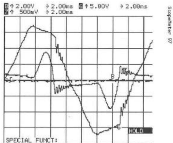
Figure 2 Voltage vs. Current – Ferro transformer
