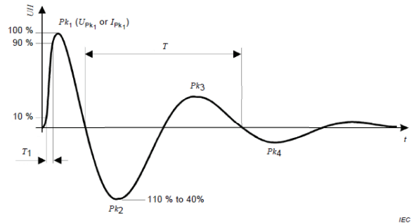
ANSI/IEEE C62.41 SWITCHING SURGES - RINGING/OSCILLATORY
